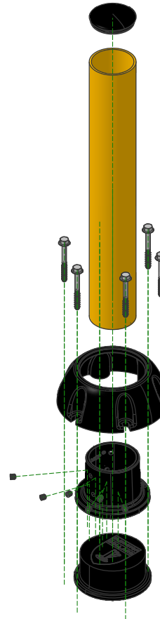
EXPLODED
